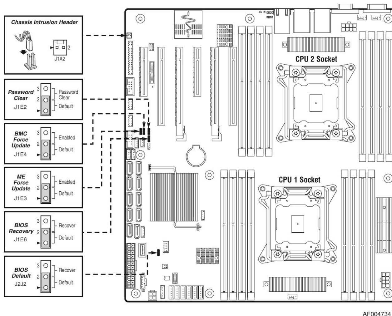
Figure 3. Jumper Block Identification
