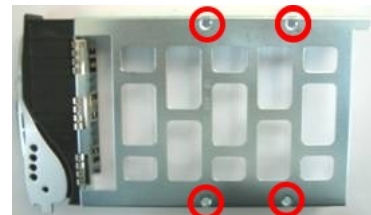
Fig. 3: Bottom view of HDD tray
