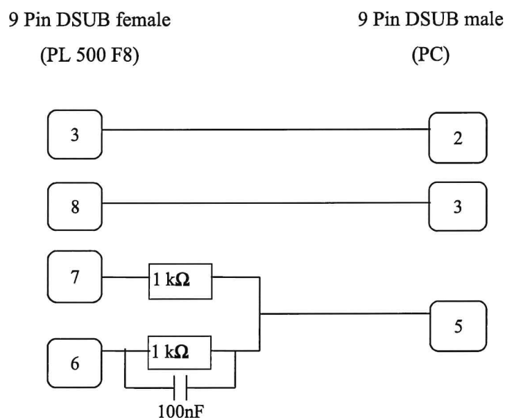
Figure 3.5: Connection of a Personal Computer
