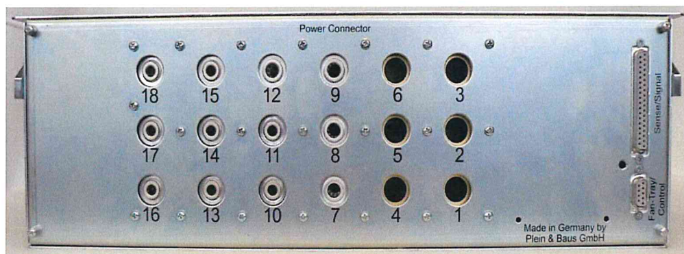
Figure 3.2: Power Box Front
