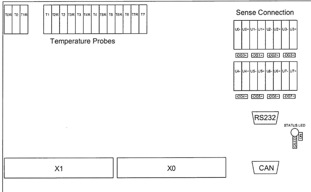
Figure 6.2: Output Register Connectors
