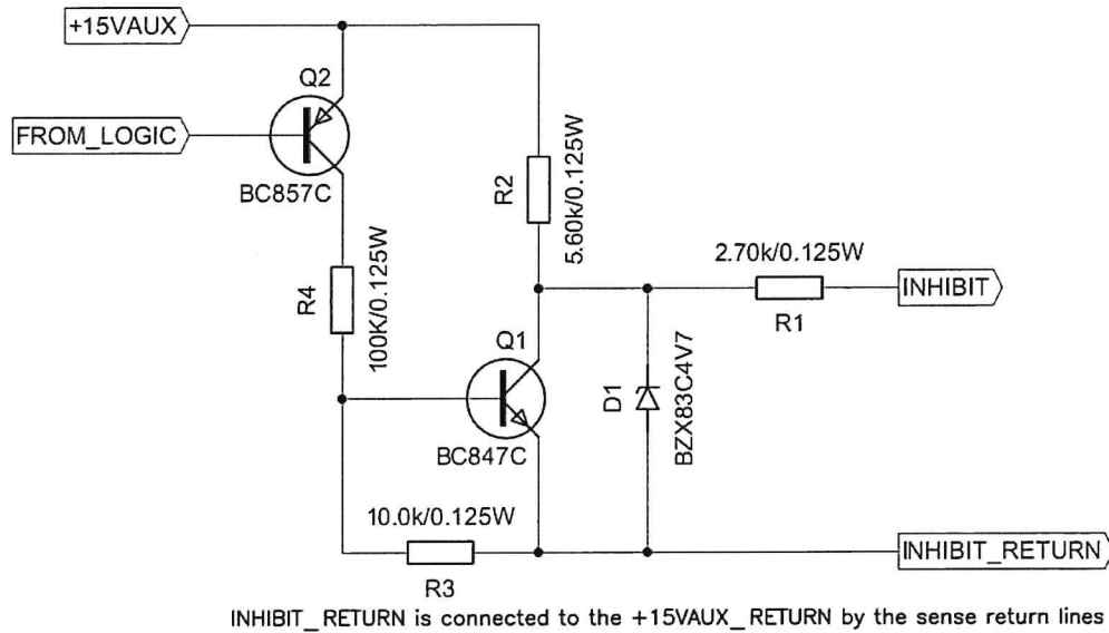
Figure 6.1: Output Register Schematic (one of 32)
