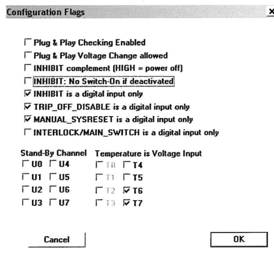
Figure 3.4: Programming of the Control Connector Behavior
