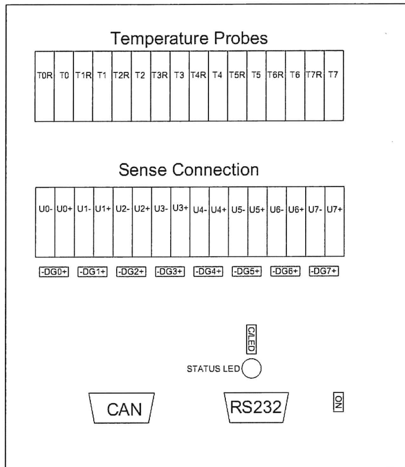
Figure 5.2: Sense Connection Connectors
