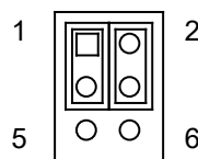
Figure 32: Backlight Power Enable Selection for LVDS1 (JP4)
