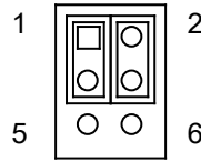
Figure 30: Panel & Backlight Power Selection for LVDS1 (JP2)
