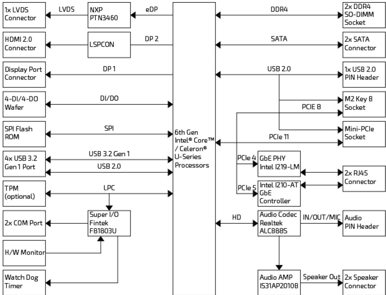
Figure 1: System Block Diagram 3.5"-SBC-SKL
