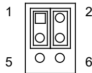
Figure 33: AT / ATX Power Mode &amp; NGFF mSATA / mPCIe Selection (JP6)
