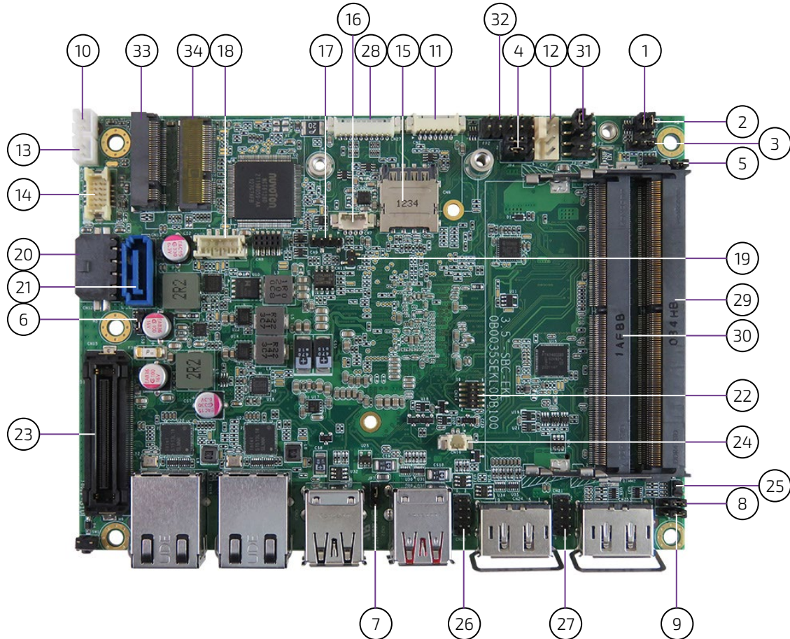
Figure 2: Top Side
