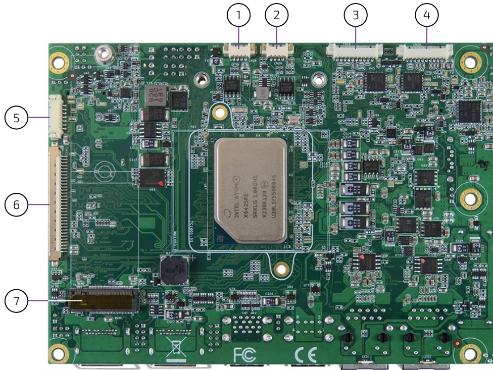
Figure 3: Rear Side
