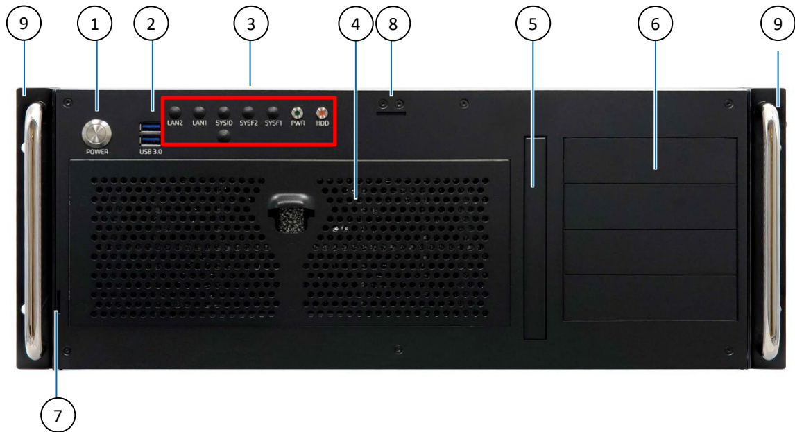
Figure 3: Front Panel
