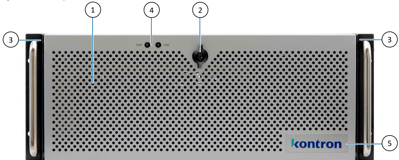
Figure 4: Front Flap
