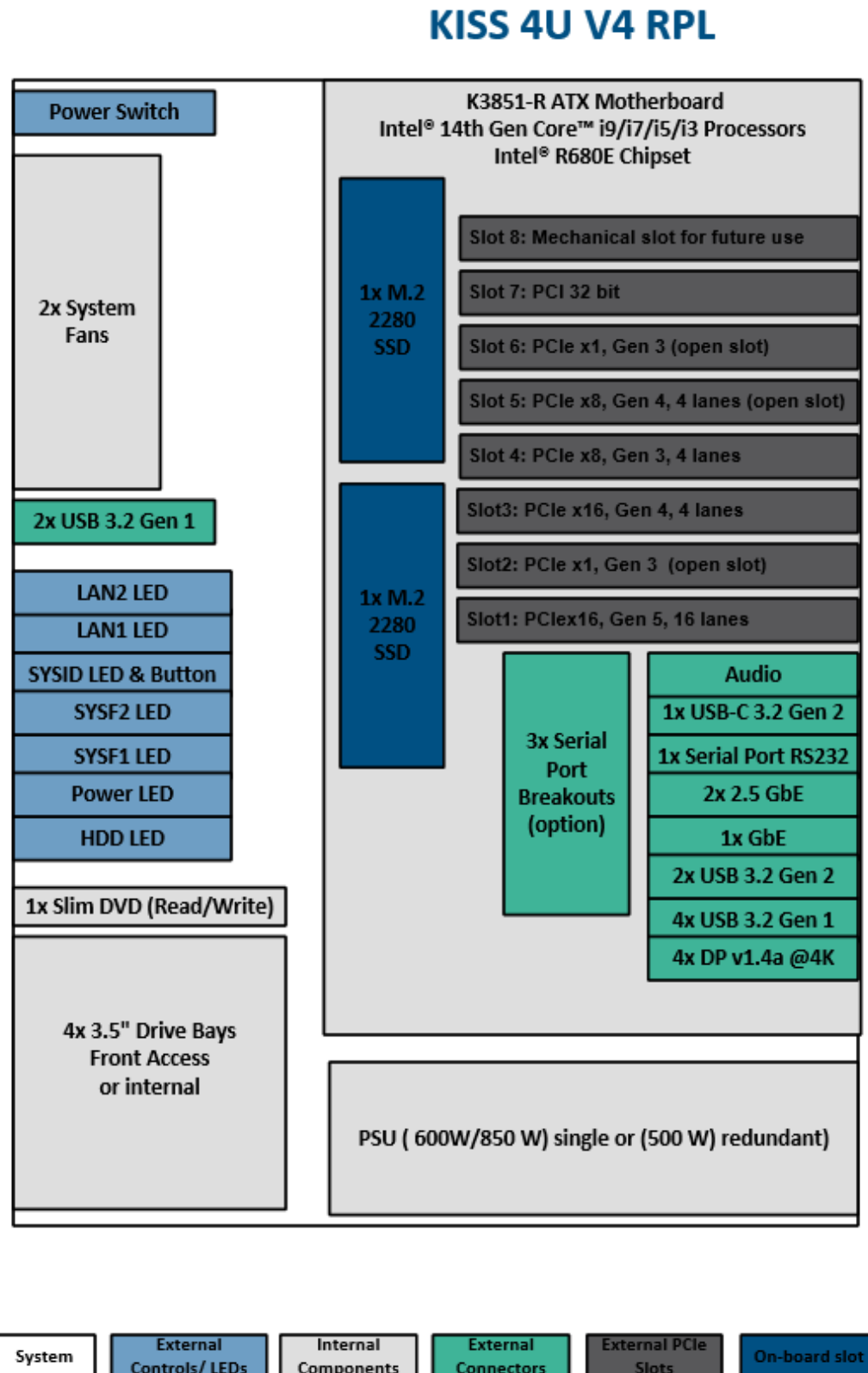
Figure 27: Block Diagram KISS 4U V4 RPL
