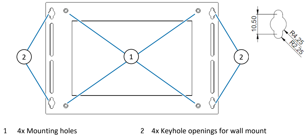
Figure 11: Wall Mount Bracket
