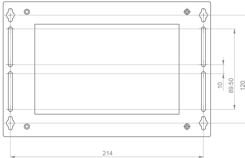
Figure 24: Wall Mount Dimensions (mm)
