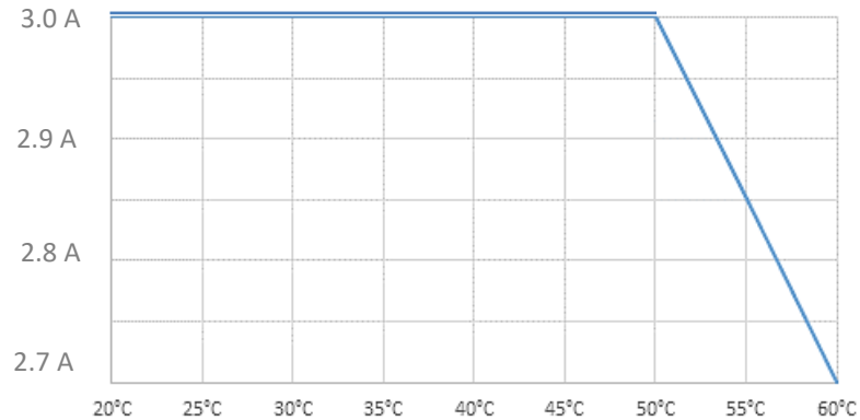
Figure 18: Derating Current USB-C Port (X102) Curve
