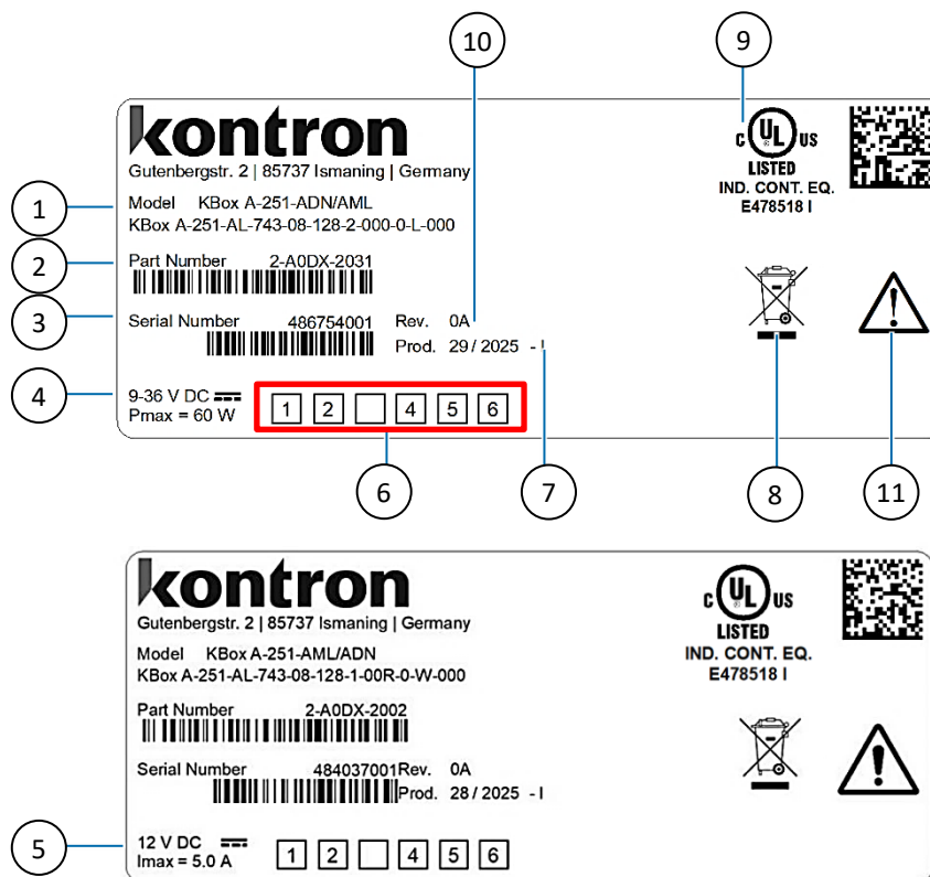
Figure 2: Type Label Example 24 VDC and 12 VDC Versions
