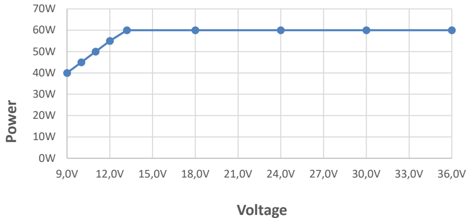
Figure 31: Voltage Power Derating (24 VDC Power Supply)
