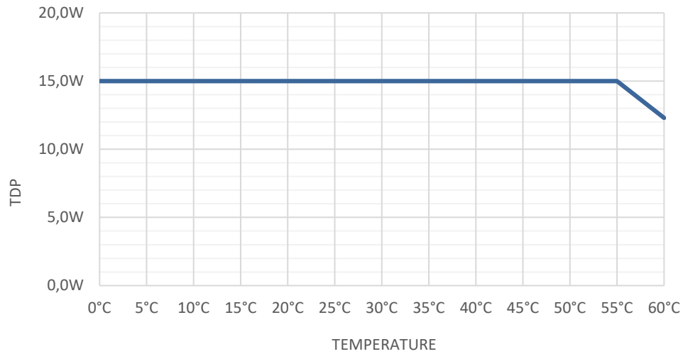
Figure 17: Derating TDP @ w/o External (USB) Load & M.2 Curve
