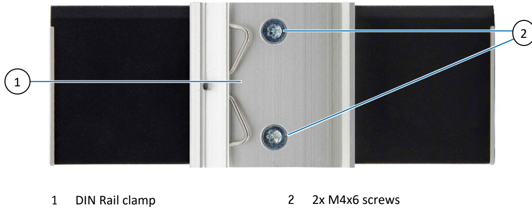
Figure 7: Rear Side
