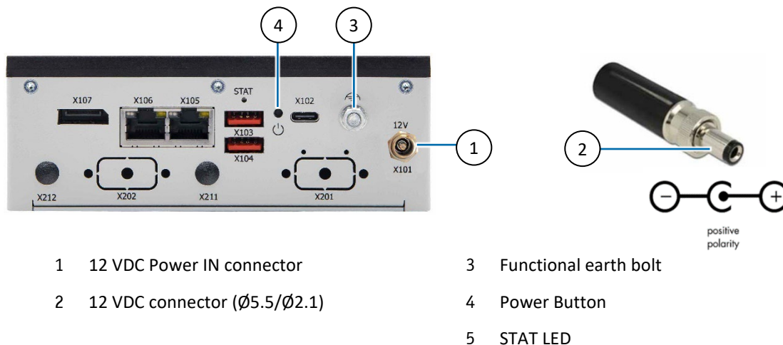
Figure 22: Power IN 12 VDC Connector and Mating Power Connector
