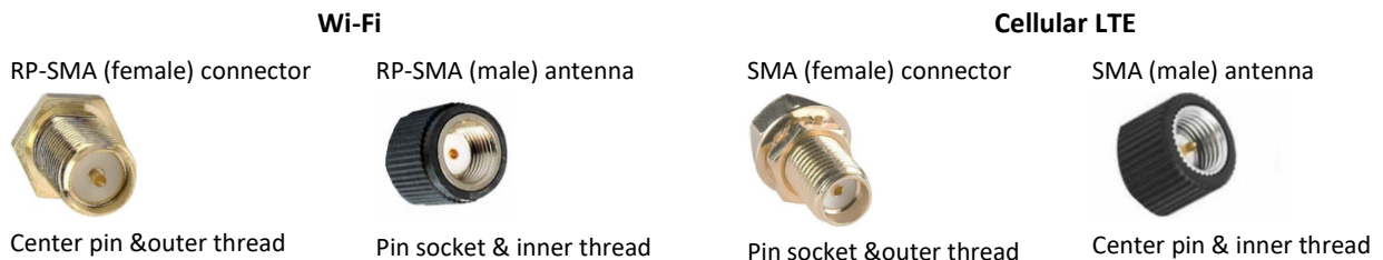
Figure 4: Wi-Fi and Cellular LTE Connectors and Antenna Type
