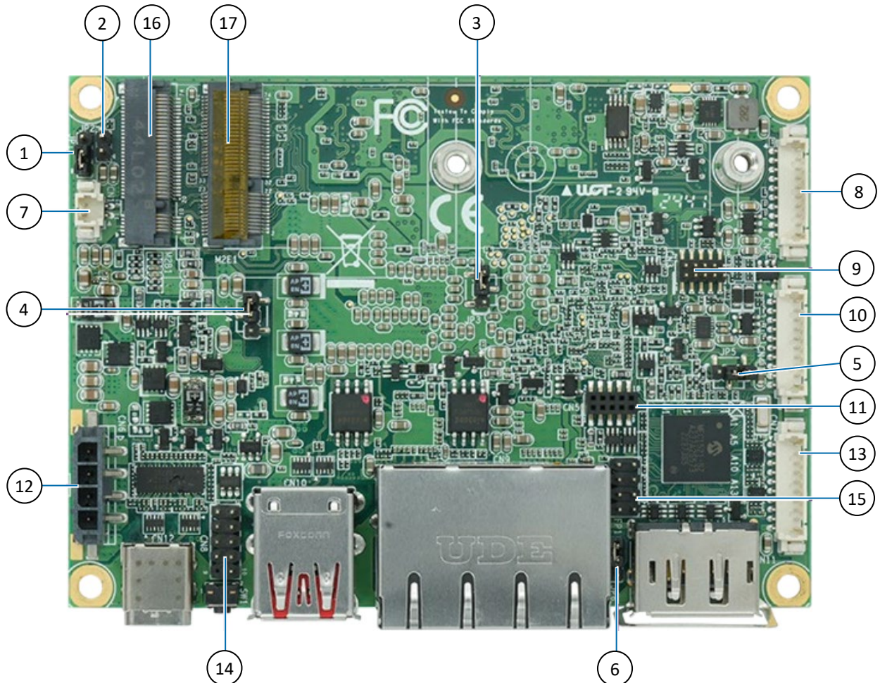
Figure 10: 2.5"-SBC-AML/ADN Onboard Components- Top Side
