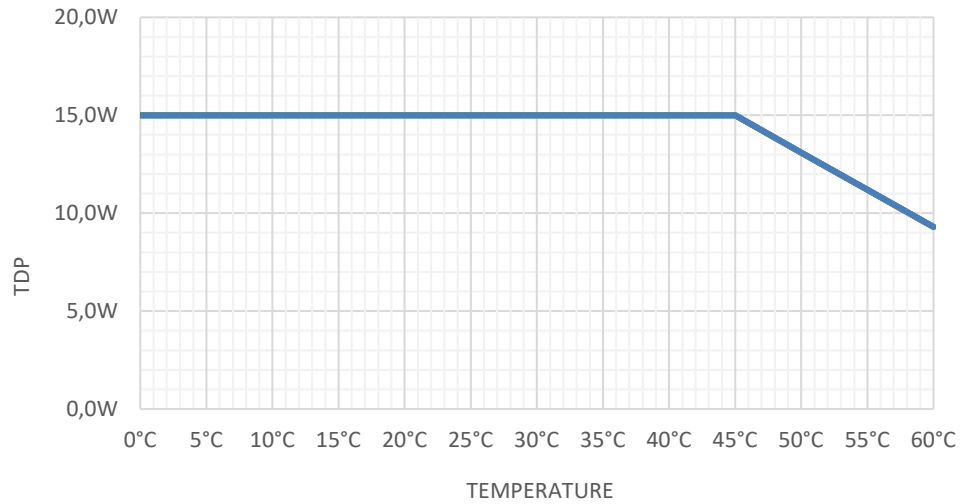
Figure 15: Derating TDP @ Absolute Max. Curve
