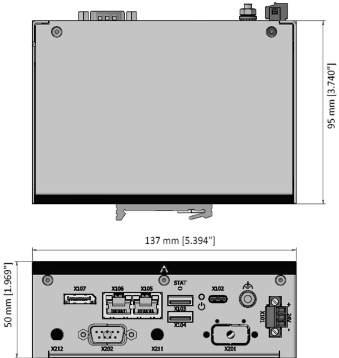
Figure 32: Mechanical Dimensions Front (mm)
