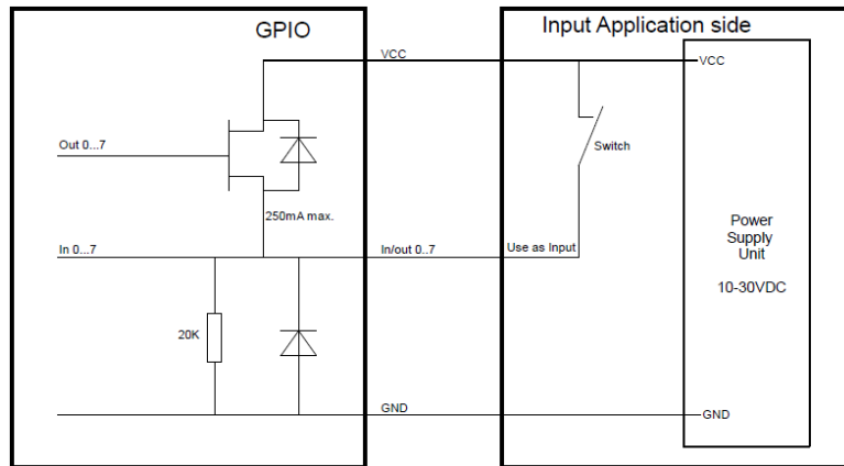
Figure 13: Input Application Connected to GPIO
