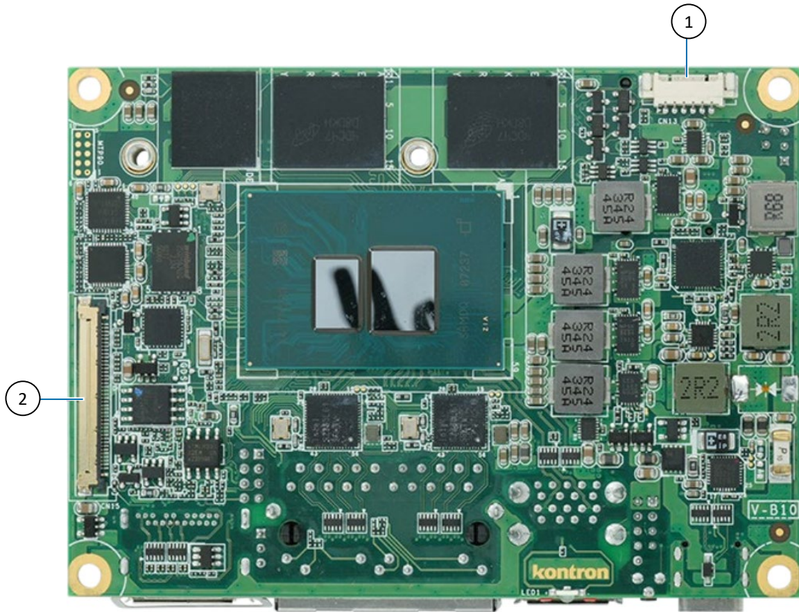
Figure 11: 2.5"-SBC-AML/ADN Onboard Components- Top Side
