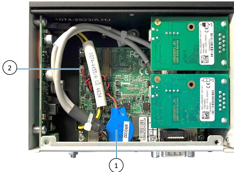
Figure 33: Lithium Battery and Battery Header
