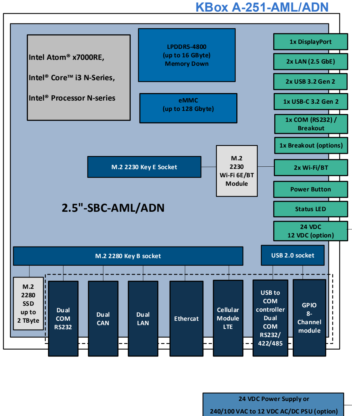
Figure 30: Block Diagram KBox A-251-AML/ADN
