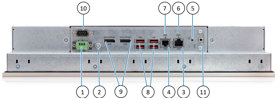
Figure 6: Interface Panel
