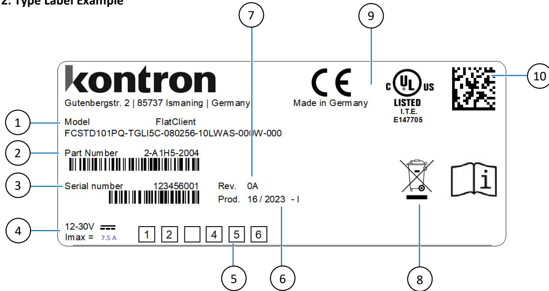
Figure 2: Type Label Example
