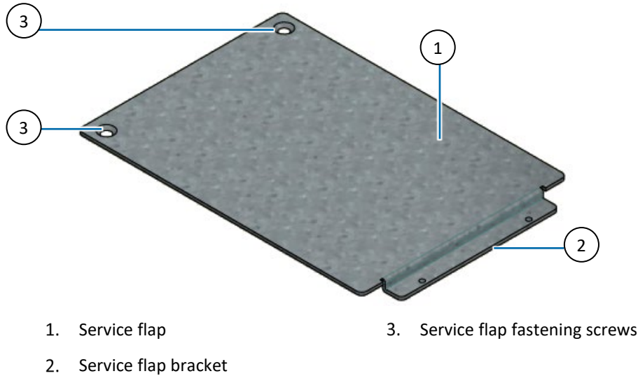
Figure 22: Automotive Battery Service Flap
