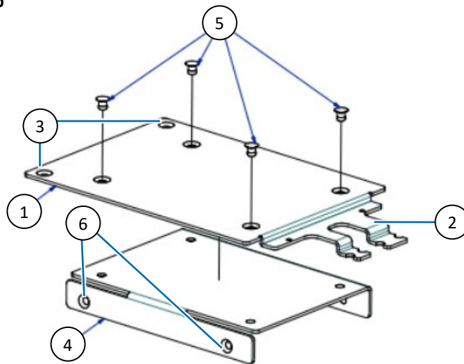
Figure 20: 2.5" SSD Service Flap
