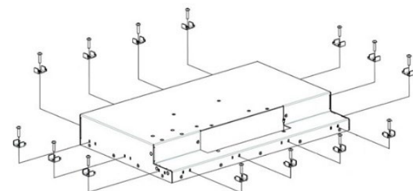
Figure 11: Clamping Bracket Positions
