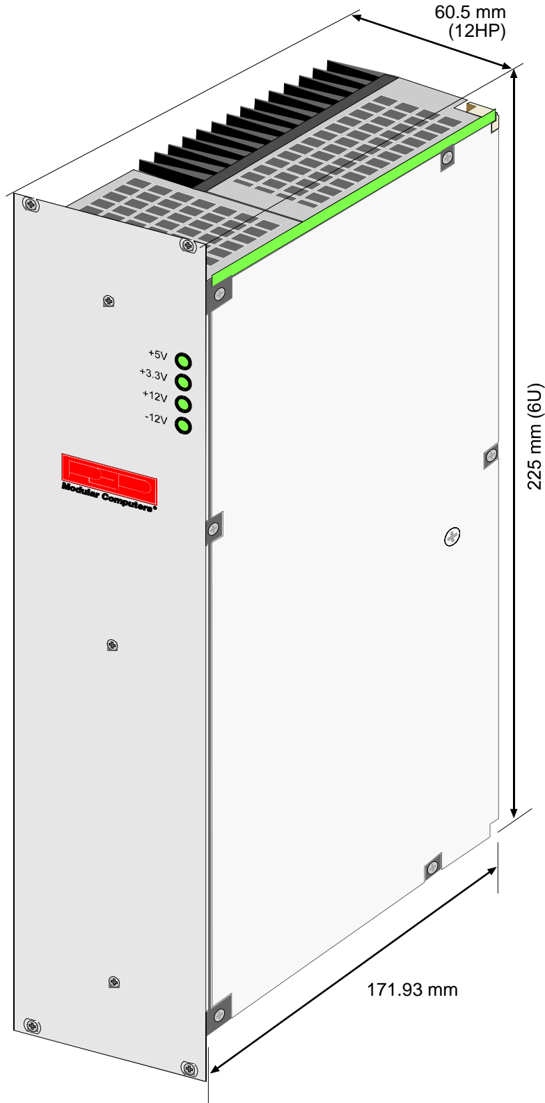
Figure 2: View of Power Supply Unit CP6-SVE-M250AC-R
