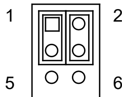
Figure 41: LVDS / eDP Backlight & Panel Power Selection JP4
