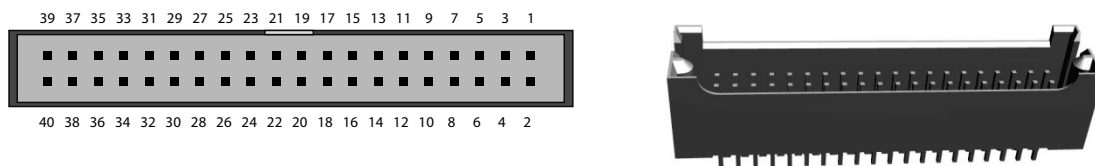
Figure 12: LVDS 40-Pin Connector
