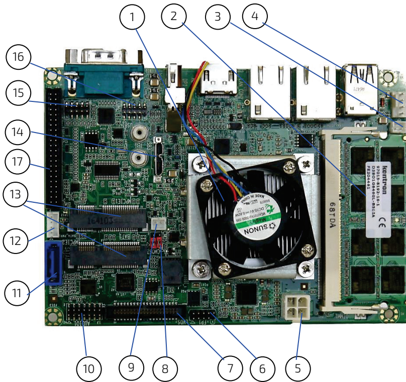
Figure 3: Top Side View
