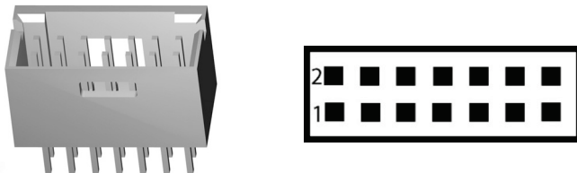
Figure 16: Audio Connector
