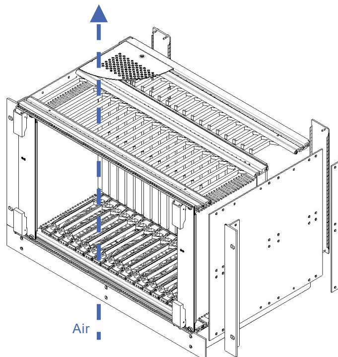
Figure 3-11: Air Flow
