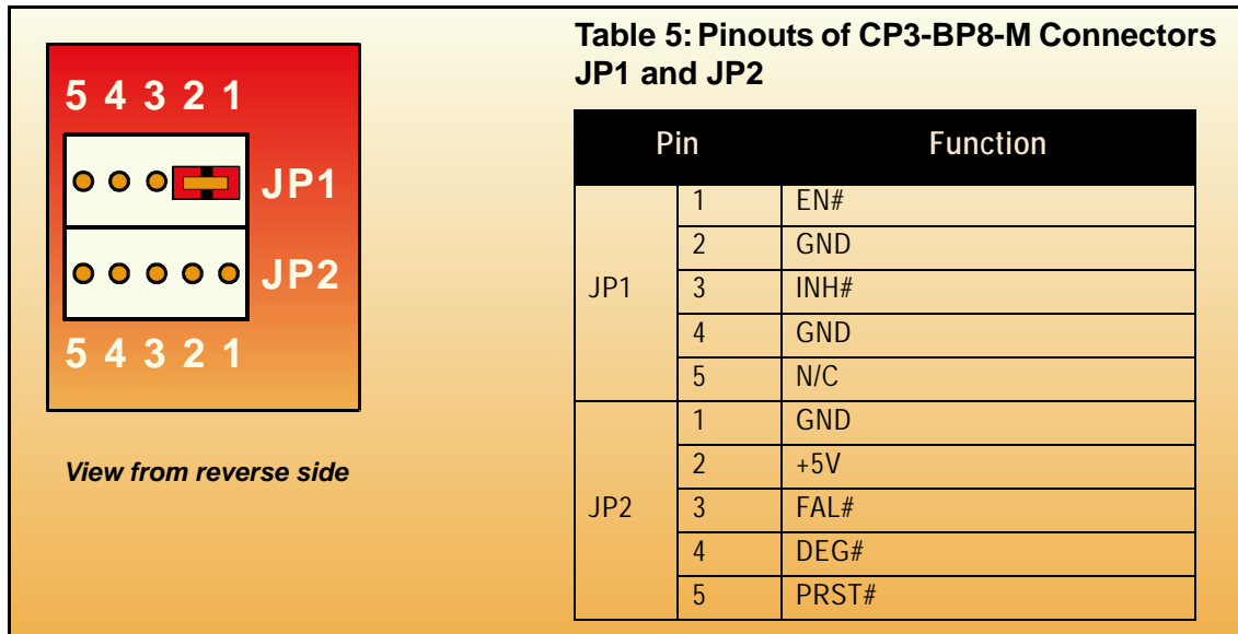
Figure 7: Orientation and Pinouts of CP3-BP8-M Connectors JP1 and JP2
