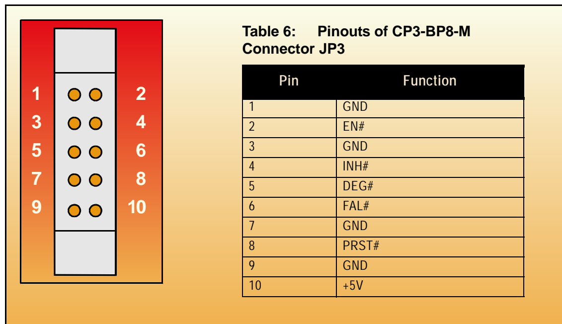
Figure 8: Orientation and Pinouts of CP3-BP8-M Connector JP3
