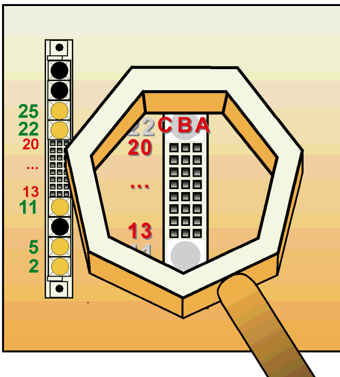
Figure 4: Orientation and Pinouts of CP3-BP8-M DIN type M Power Supply Connector
