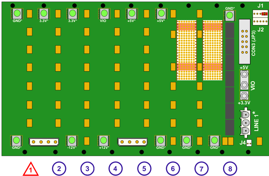
Figure 2: CP3-BP8-M Board Layout (Reverse)
