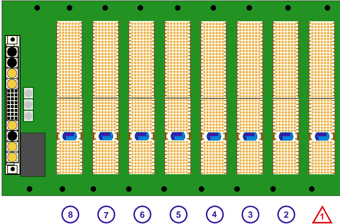
Figure 2: CP3-BP8-M Board Layout (Reverse)
